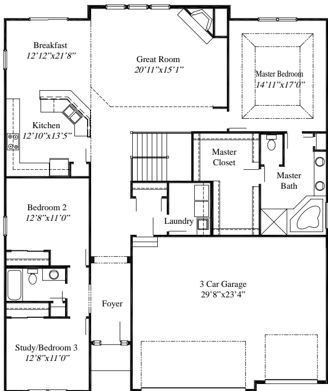
First Floor 2,130 sq ft
