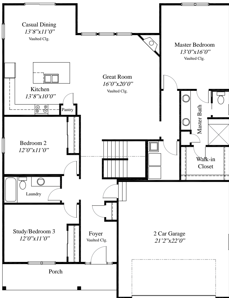
First Floor 1,743 sq ft
